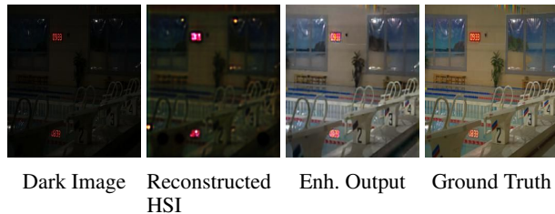
Figure 1: A sample dark image along with the reconstructed HSI and the output obtained using SpecNet. SpecNet produces output very close to the ground truth in terms of color and details, as can be seen by comparing with the ground truth image SPECNET.
